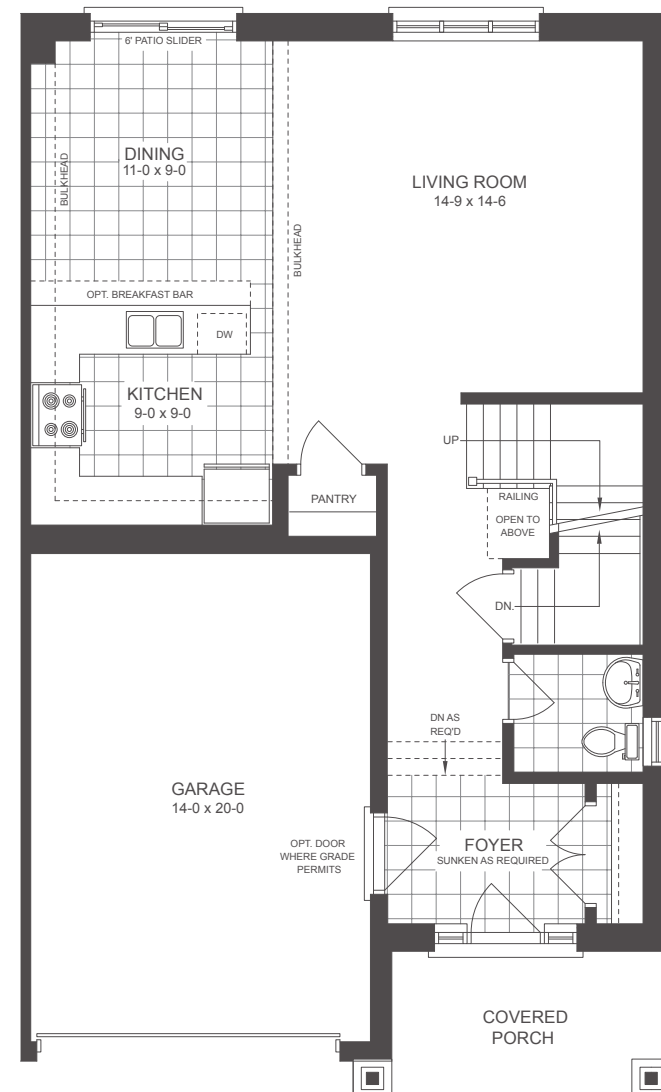
MAIN FLOOR
