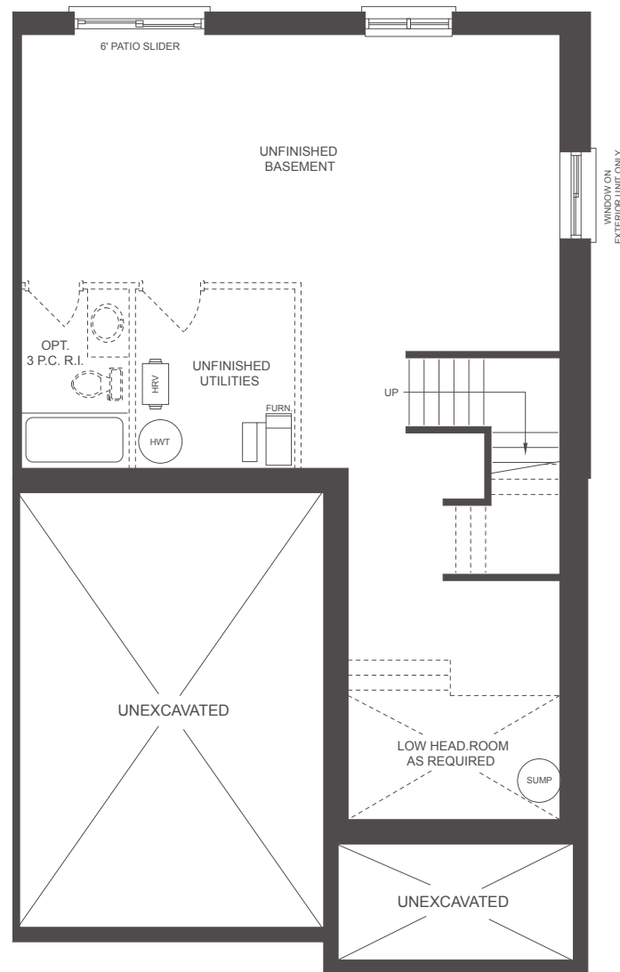
BASEMENT
